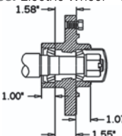
A-HS276066HK Hub Kit L/Spindle
