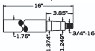
A-SP25005 Spindle
