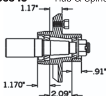
A-HS1750545 Hub & Spindle Assy. (5 Bolt)
