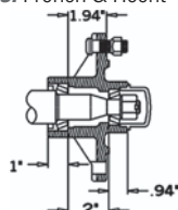
A-HS20006S6HK Hub Kit L/Spindle
