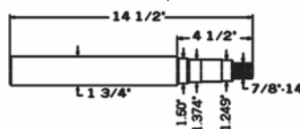
A-SP2760 Spindle
