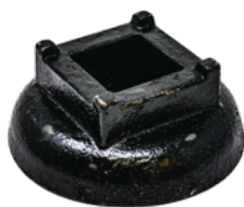
A-VLH6706 Washer, Large For 1" Axles, Cast Iron, Painted Black A: 6.437" B: 1.750" C: 1.062" D: 1.125"
