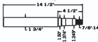
A-SP2760 Spindle
