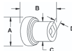
A-VLH6709 Spool Spacer 3-5/8" For 1" Axle, Cast Iron, Painted Black A: 3" B: 3.312" C: 2.250" D: 1.000"
