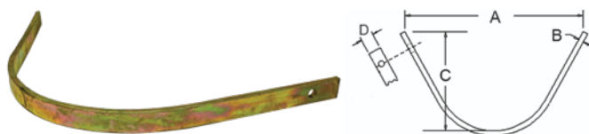
A-RRT1 Rock Rake Tooth .375" mounting hole A - 17" B - .315" C - 9 5/8" D - 1"
