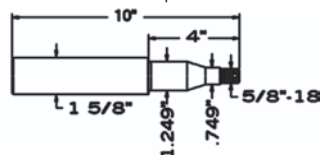
A-SP2000 Spindle
