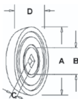
A-VLH6706 Washer, Large For 1" Axles, Cast Iron, Painted Black A: 6.437" B: 1.750" C: 1.062" D: 1.125"
