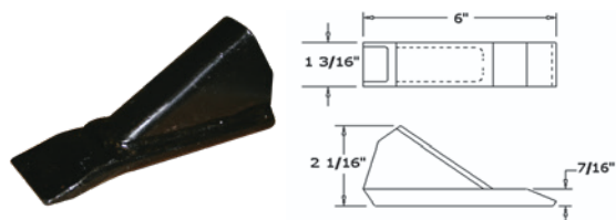
A-BSP8075 Box Scraper Point
