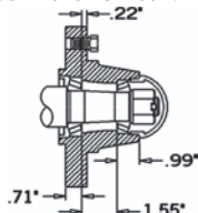
A-HS2500555HK Hub Kit L/Spindle
