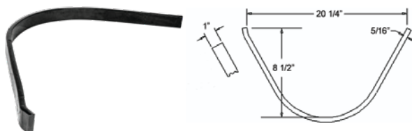
A-ELSR06 Landpride Landscape Rake Tine A - 20 1/4" B - 5/16" C - 8 1/2" D - 1"
