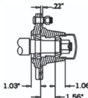
A-HS27605S55HK Hub Kit L/Spindle
