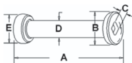
A-VLH6704 Plain Spool 7 1/2" For 1" Axles, Cast Iron, Painted Black A: 7.434" B: 4" C: 1.062" D: 2" E: 3"
